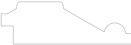
3551 Base cap 0.875" x 2.687"
