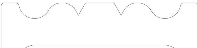
1070 Casing 0.812" x 3.500"
