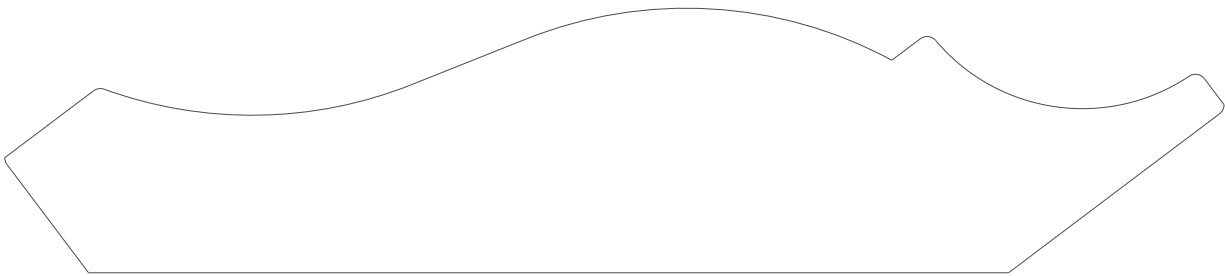
2575 Crown 1.378" x 6.351"
