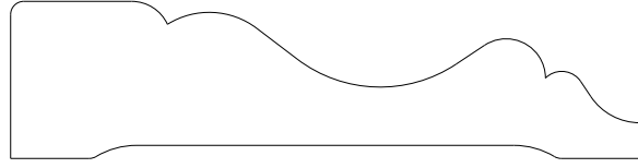
1022 Casing 0.750" x 3.000"
