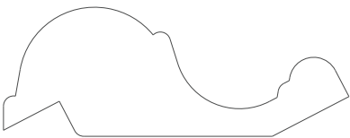
8550 Panel mold 0.750" x 2.000"
