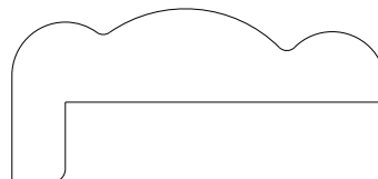
7577 Molding 0.812" x 1.750"
