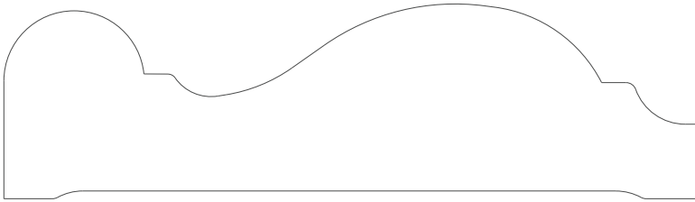
1577 Casing 1.125" x 4.000"
