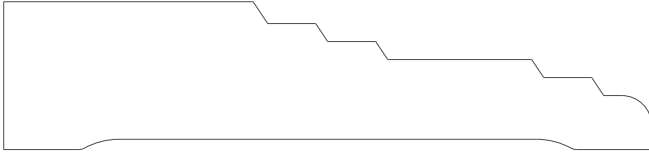
1534 Casing 0.750" x 3.375"
