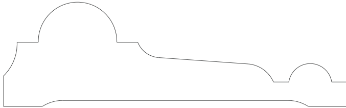
4528 Chair rail 1.062" x 3.500"
