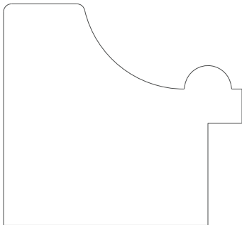
1580 Backband 1.625" x 1.750"
