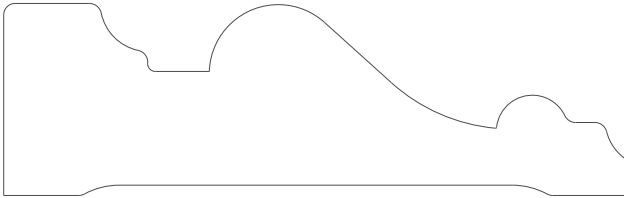
1078 Casing 1.000" x 3.250"
