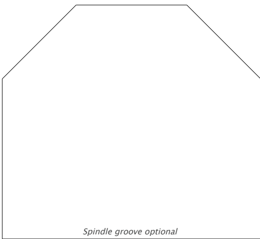
4320 Handrail 2.375" x 2.625"
