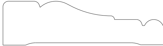
1025 Casing 0.750" x 2.750"
