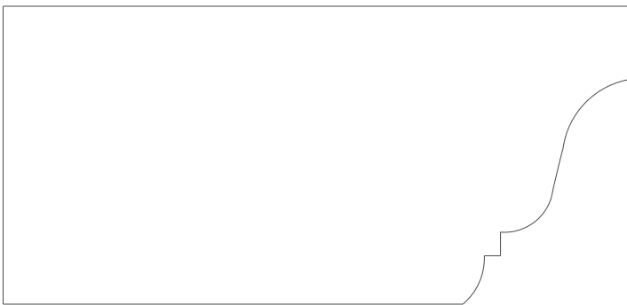
2018 Crown 1.750" x 3.687"
