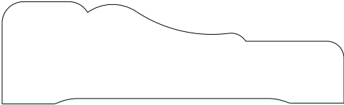
1017 Casing 0.750" x 2.500"
