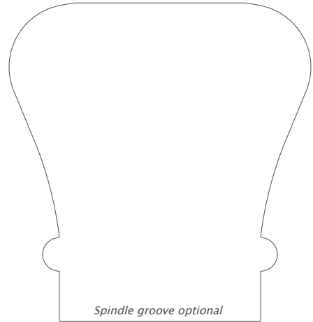
4057 Handrail 2.375" x 2.250"
