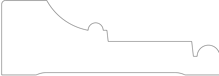
1570 Casing 1.250" x 3.625"
