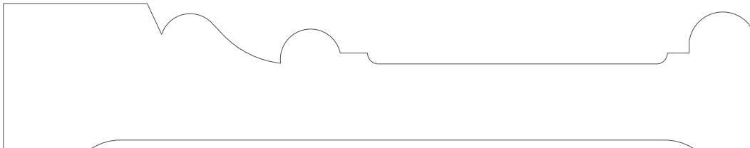
1562 Casing 1.062" x 5.500"
