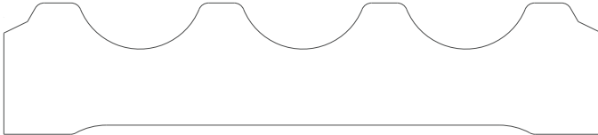
1541 Casing 0.750" x 3.500"
