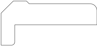
7578 Molding 0.812" x 1.750"
