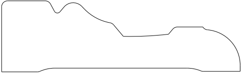
1529 Casing 0.750" x 2.500"
