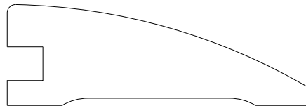
7626 Threshold 0.750" x 2.250"
