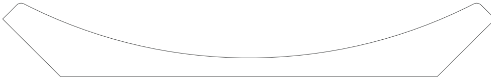
2559 Crown 0.750" x 5.000"
