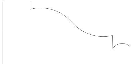
8581 Panel mold 1.125" x 2.368"
