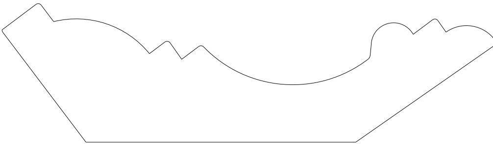
2580 Crown 1.478" x 5.250"
