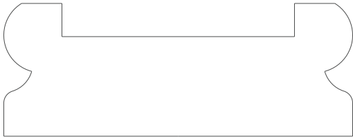
4555 Shoe 1.000" x 2.625"
