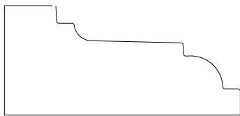
7573 Molding 0.812" x 1.750"
