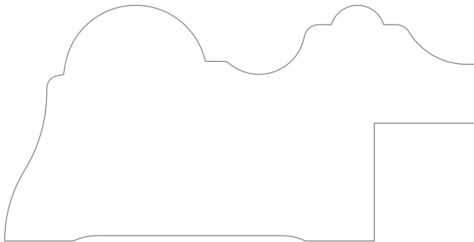
4530 Chair rail 1.750" x 3.500"
