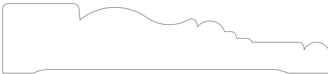
1059 Casing 0.750" x 3.500"
