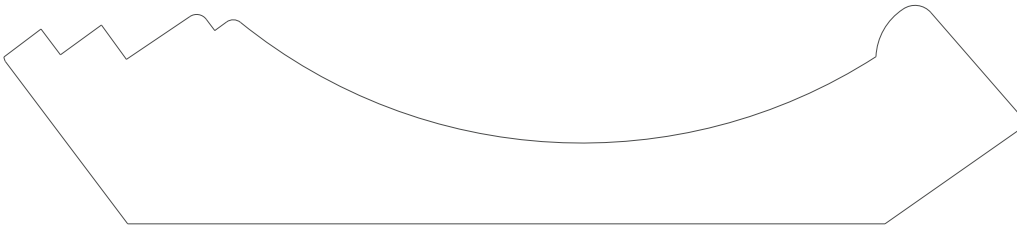
2563 Crown 1.090" x 5.315"
