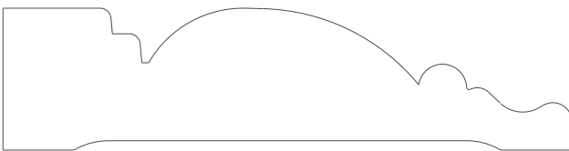
1567 Casing 0.812" x 3.250"
