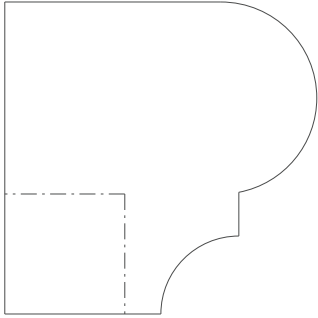
4585 Nosing 1.625" x 1.625"
