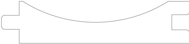
5503 Planking 0.750" x 3.312"
