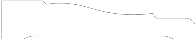
1004 Casing 0.687" x 3.500"
