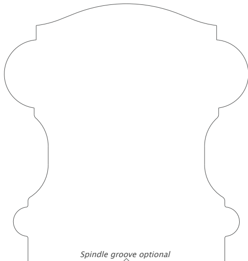
4595 Handrail 2.750" x 2.625"
