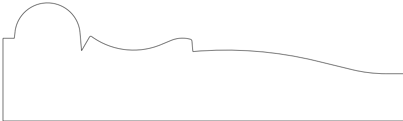
7592 Molding 1.250" x 4.250"
