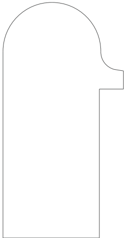
4561 Nosing 1.125" x 2.443"
