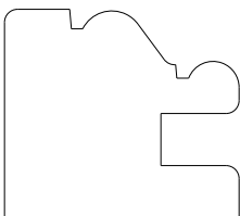
7513 Molding 1.000" x 1.125"
