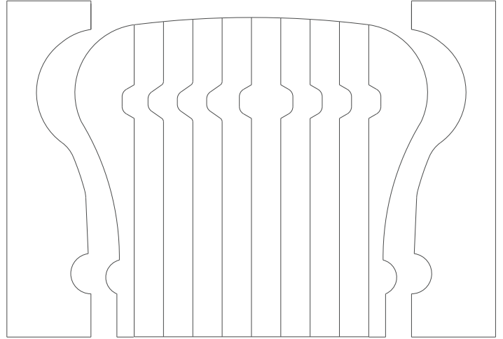
4593B Handrail 2.375" x 2.625"
