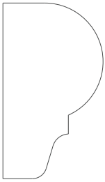
4085 Nosing 0.750" x 1.312"
