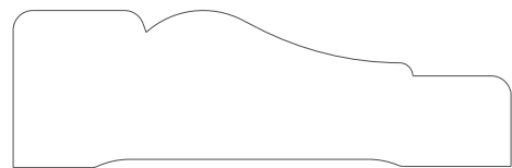
1015 Casing 0.750" x 2.375"
