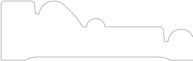
1246 Casing 1.000" x 3.250"
