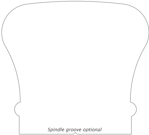
4593 Handrail 2.375" x 2.625"
