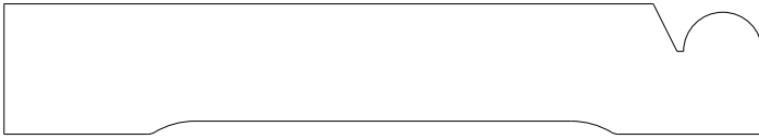
1227 Casing 0.625" x 3.625"
