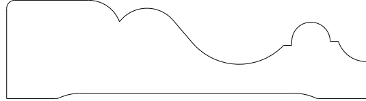
1023 Casing 0.750" x 2.750"
