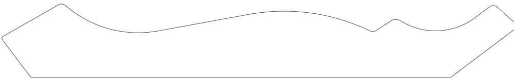
2051 Crown 0.750" x 5.250"
