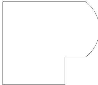
4575 Nosing 1.500" x 1.750"
