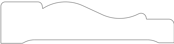
1035 Casing 0.750" x 3.125"
