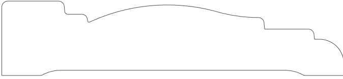
1569 Casing 0.750" x 3.500"
