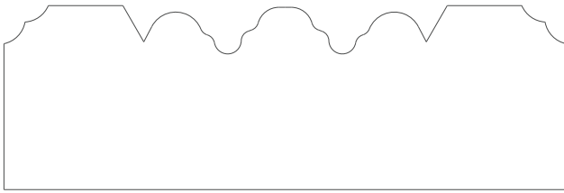
1572 Rosette 1.062" x 3.250"
