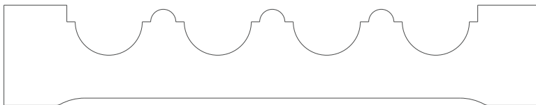
1558 Casing 0.750" x 4.000"
