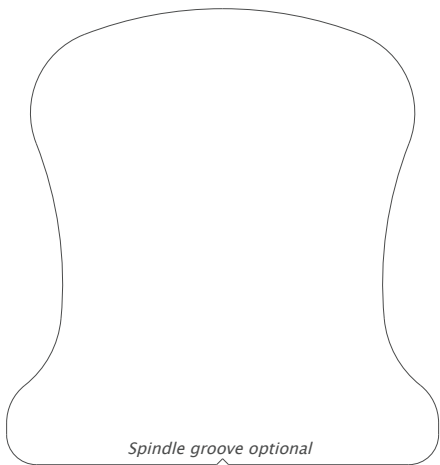
4557 Handrail 2.375" x 2.250"
