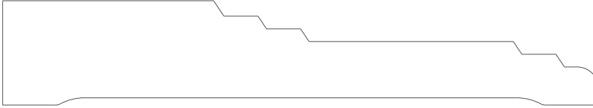
1535 Casing 0.750" x 4.375"
