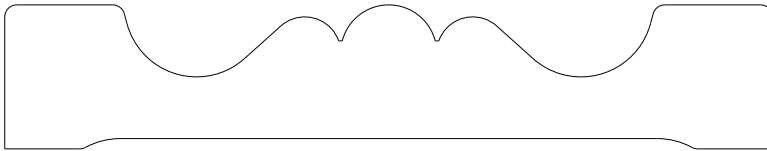
1050 Casing 0.750" x 4.000"
