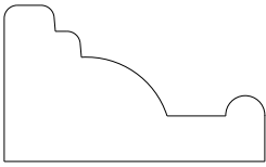
7521 Molding 0.750" x 1.125"
