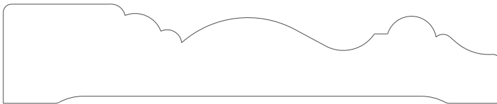
1538 Casing 0.750" x 3.750"
