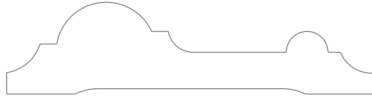
4520 Chair rail 0.687" x 2.750"
