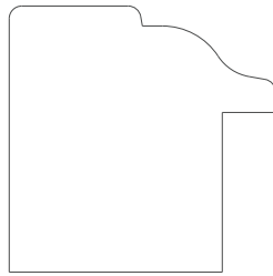
1041 Backband 1.250" x 1.250"
