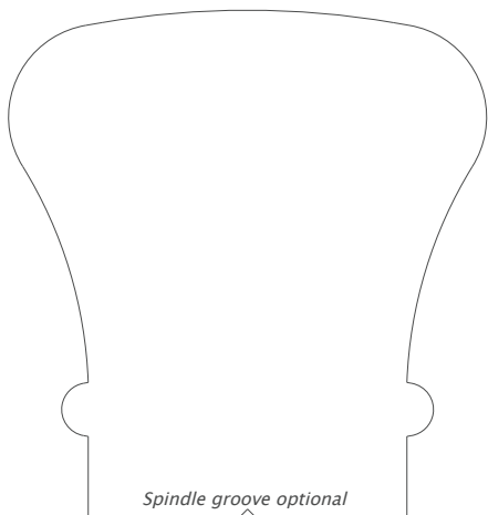
4592 Handrail 2.375" x 2.250"
