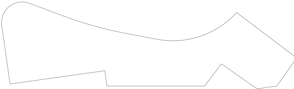
2572 Crown 1.449" x 5.391"
