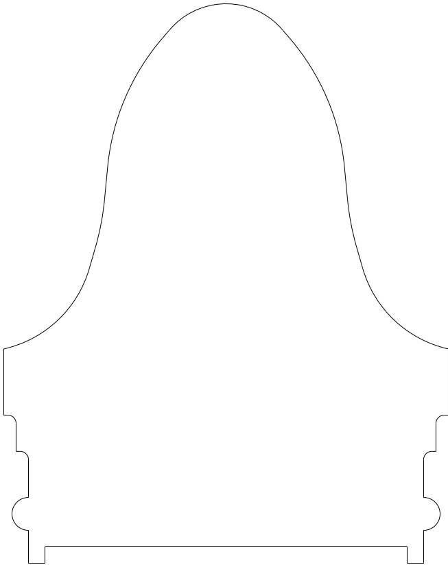
4574 Handrail 4.250" x 3.375"
