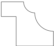
7596 Molding 0.750" x 0.875"
