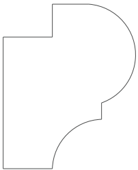
4586 Nosing 1.000" x 1.125"
