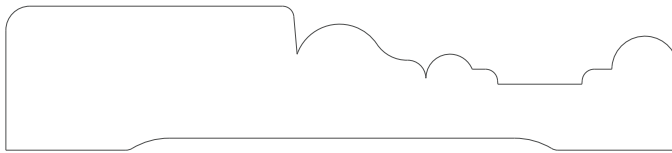
1561 Casing 0.750" x 3.500"
