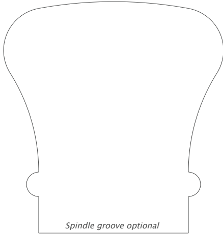
4050 Handrail 2.375" x 2.250"
