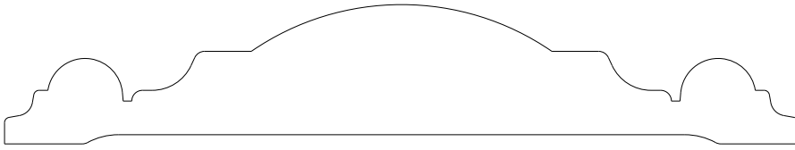
7570 Molding 0.812" x 4.625"
