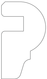
4086 Edgeband 0.750" x 1.312"
