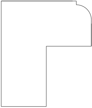
7559 Molding 1.750" x 1.500"
