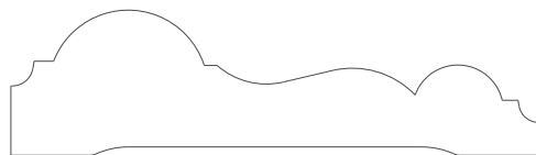
4098 Chair rail 0.687" x 2.500"
