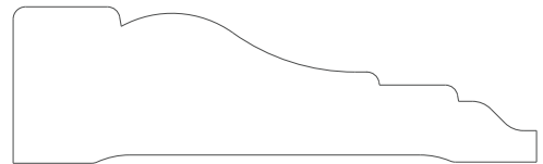
1014 Casing 0.750" x 2.500"
