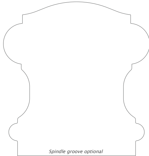
4546 Handrail 2.750" x 2.625"
