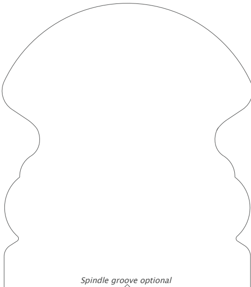
4594 Handrail 3.000" x 2.625"
