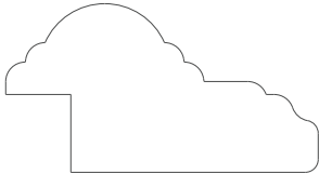
8020 Panel mold 0.812" x 1.500"
