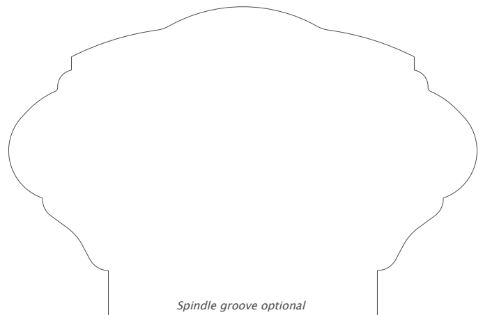
4558 Handrail 2.312" x 3.500"
