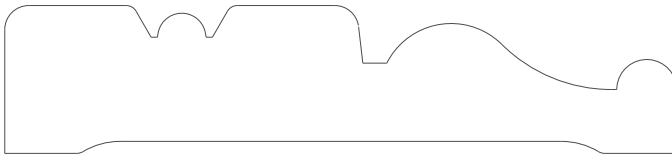
1537 Casing 0.750" x 3.500"
