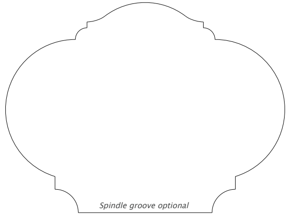
4553 Handrail 2.250" x 3.000"
