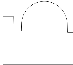
7568 Molding 1.100" x 1.250"
