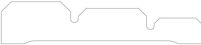
1130 Casing 0.750" x 3.500"
