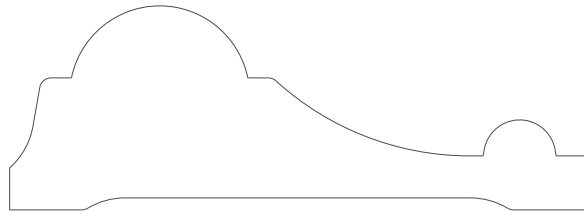
4522 Chair rail 1.062" x 3.000"
