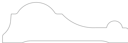
4523 Chair rail 0.812" x 2.500"
