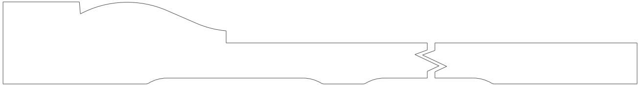
3084 Base 0.875" x 7.250"
