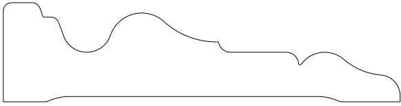
1028 Casing 0.750" x 3.000"
