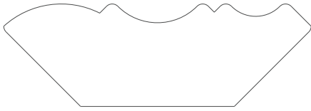
2520 Crown 0.750" x 2.250"
