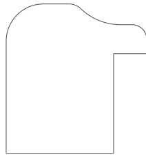
1509 Backband 1.125" x 1.062"
