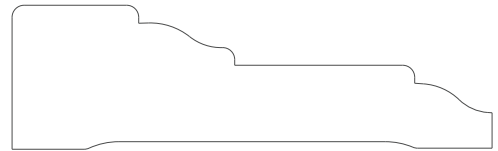
1013 Casing 0.750" x 2.500"
