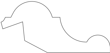
8547 Panel mold 0.904" x 1.943"
