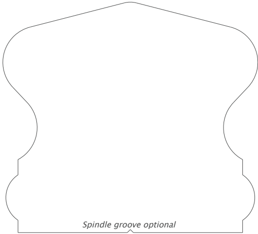
4596 Handrail 2.375" x 2.625"
