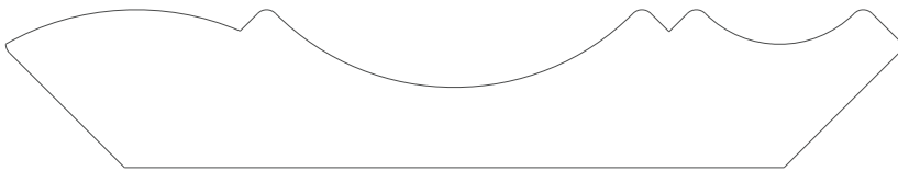
2540 Crown 0.750" x 4.250"
