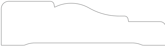
1016 Casing 0.750" x 2.750"
