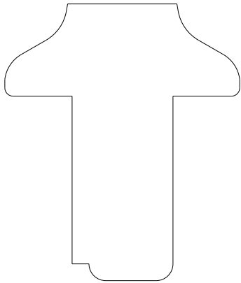
7010 Astragal 2.062" x 1.750"
