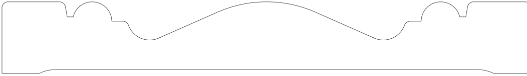
1559 Casing 0.750" x 5.500"
