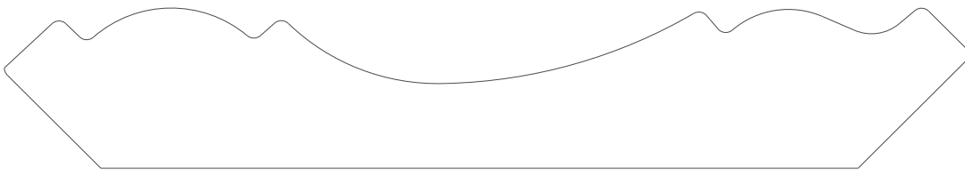
2555 Crown 0.937" x 5.625"
