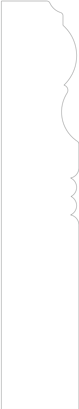
3525 Plinth 1.375" x 7.250" x 3.750"
