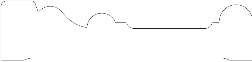
1564 Casing 1.000" x 4.250"
