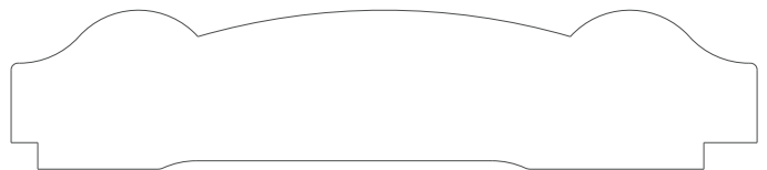
4079 Chair rail 0.750" x 3.500"
