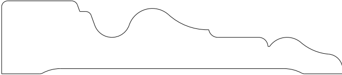
1042 Casing 0.750" x 3.500"
