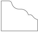
7585 Molding 0.625" x 0.750"
