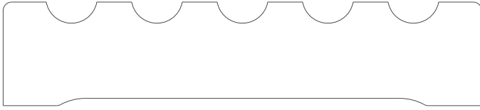
1429 Casing 0.750" x 3.500"
