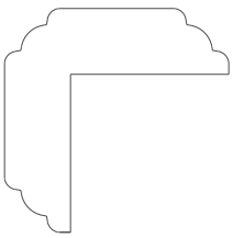
2847 Corner mold 1.062" x 1.062"
