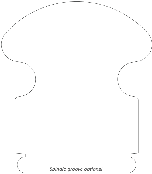
4250 Handrail 3.125" x 2.750"
