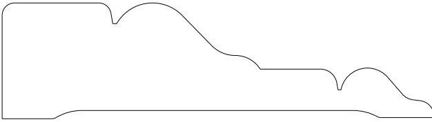
1033 Casing 0.875" x 3.250"
