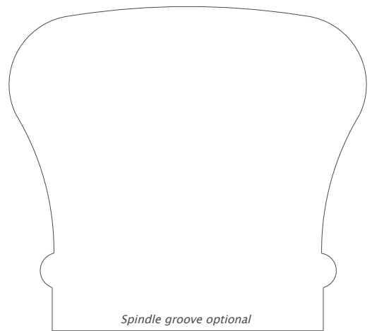
4059 Handrail 2.375" x 2.625"
