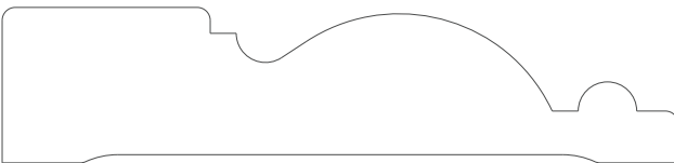
1527 Casing 0.750" x 3.250"
