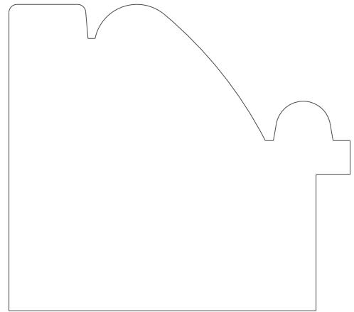
1690 Backband 2.250" x 2.500"
