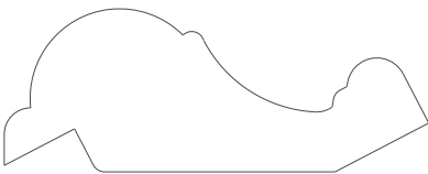
8549 Panel mold 0.750" x 2.000"
