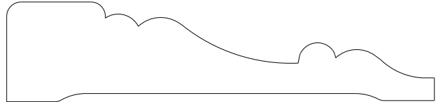
1026 Casing 0.750" x 3.250"
