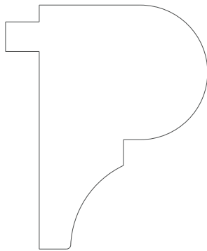
4579 Nosing 1.812" x 1.500"
