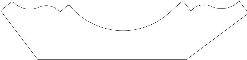
2579 Crown 1.062" x 4.500"
